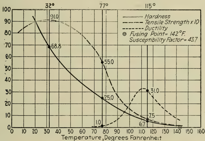
FIG. 45.—Chart of Physical Characteristics of Fluxed Gilsonite Mixture.
